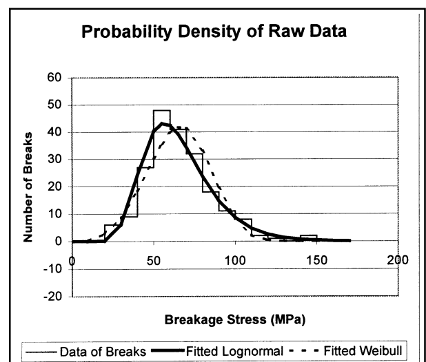
Figure 1. Comparison between the Weibull & Log normal distributions.
