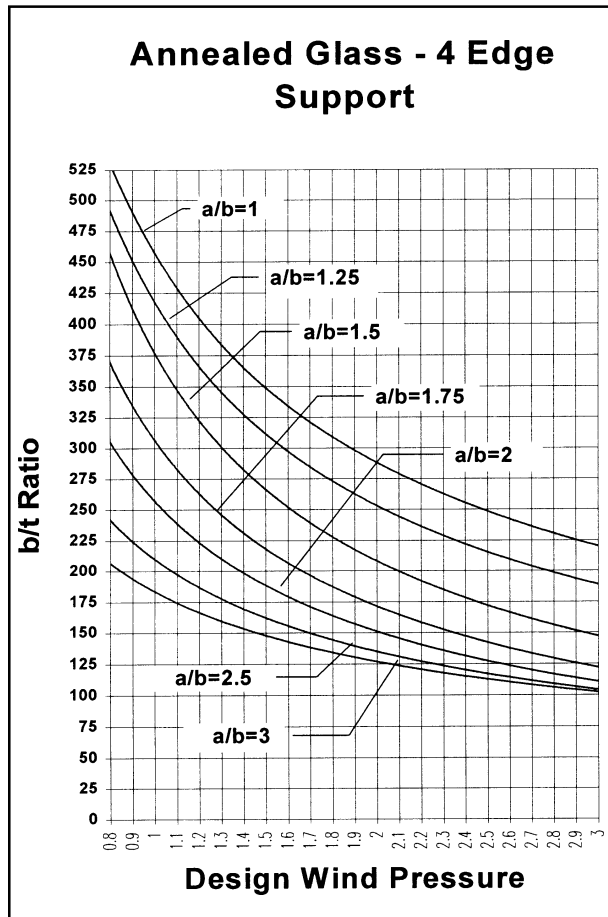
Figure 4. New Design Chart - Ultimate Limit State Loading.
