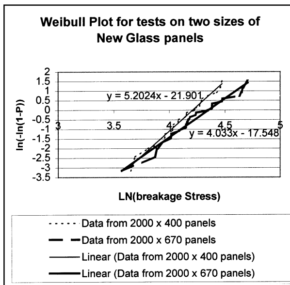
Figure 2. Weibull Plot for new Glass.
