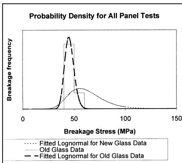
Figure 3. Breakage Data for 30 Year Old Glass.
